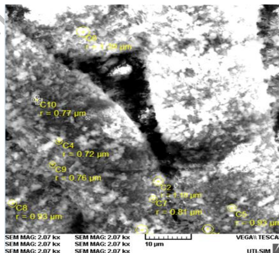
SEM image of the filter for identification of micron and submicron particles retained on the filter
