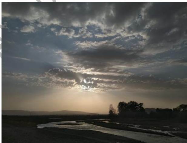
The atmosphere loaded with dust particles, on August 24 th , 2022 at 15:51 UTC, in the area of the city of Târgu Neamț, Neamț county, on the banks of the Ozana river (photo: Adrian Timofte)
