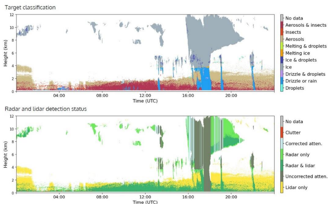
Cloudnet image from UGAL – REXDAN - Galați, combining radar and lidar data 47
